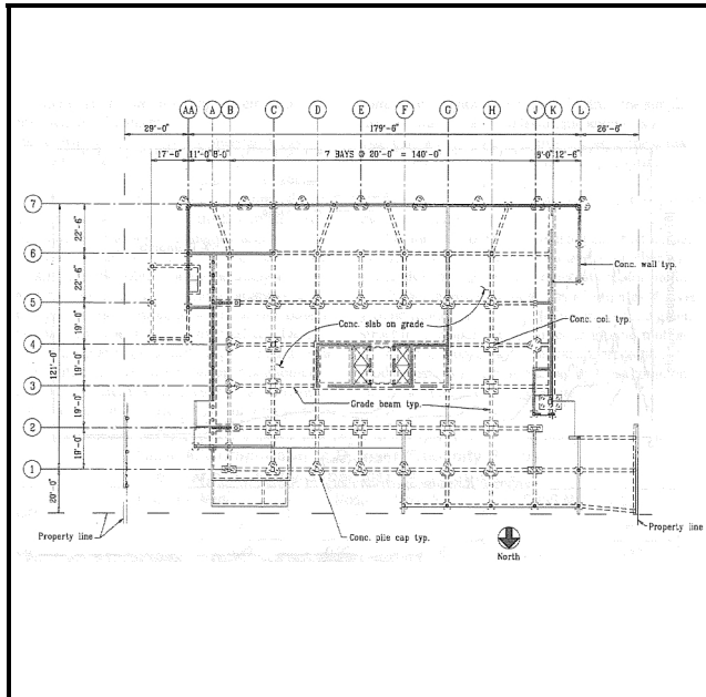
Foundation and first floor framing plan. (SSC, 1996)
