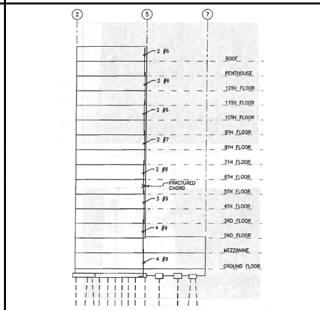
Wall elevation along Line K. (SSC, 1996)
