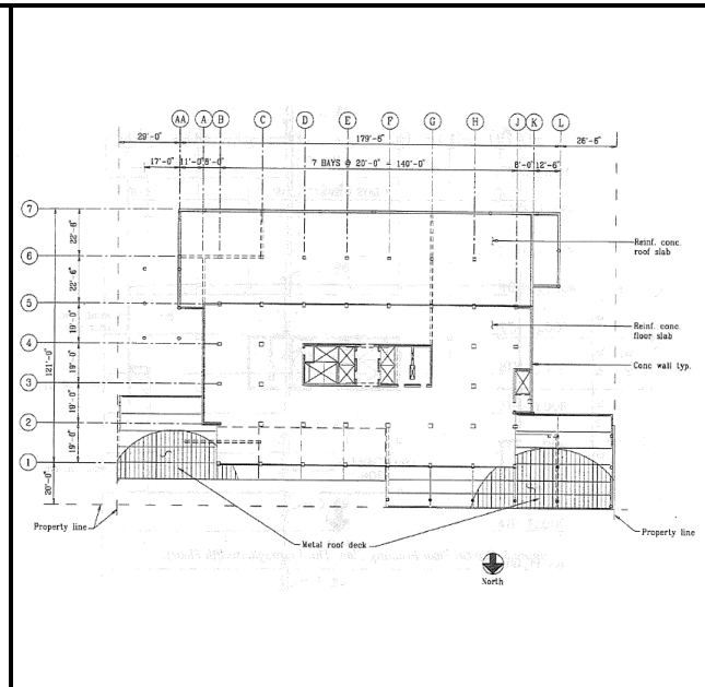
Second floor and low roof framing plan. (SSC, 1996)
