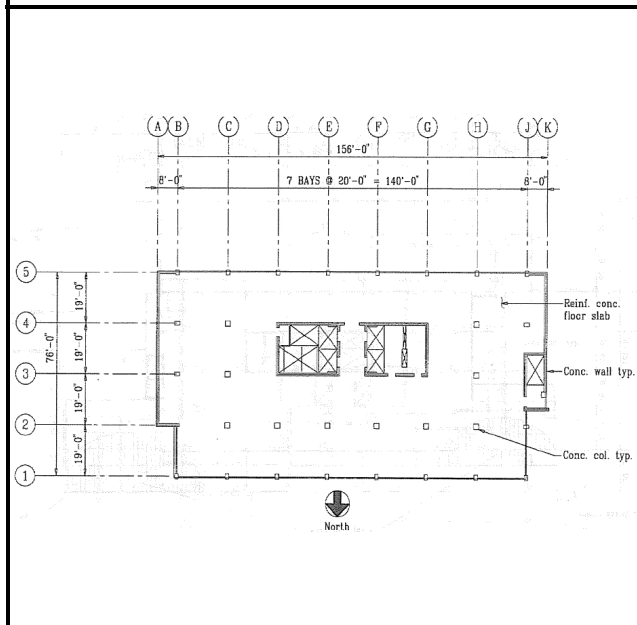
Typical floor framing plan (third through twelfth floor). (SSC, 1996)
