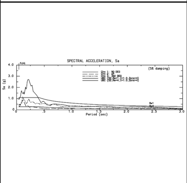
Spectral acceleration at CSMIP Station No. 24538. (CESMD, 1994)
