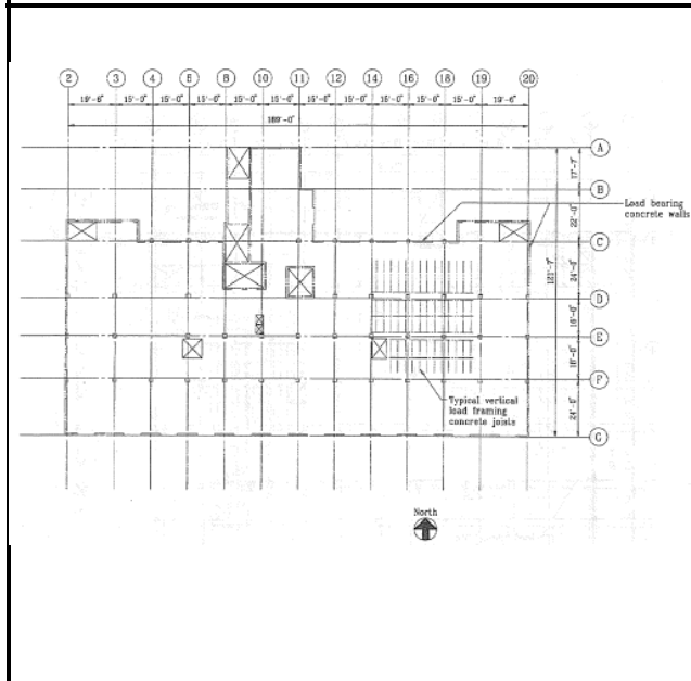
Typical floor plan. (SSC, 1994)
