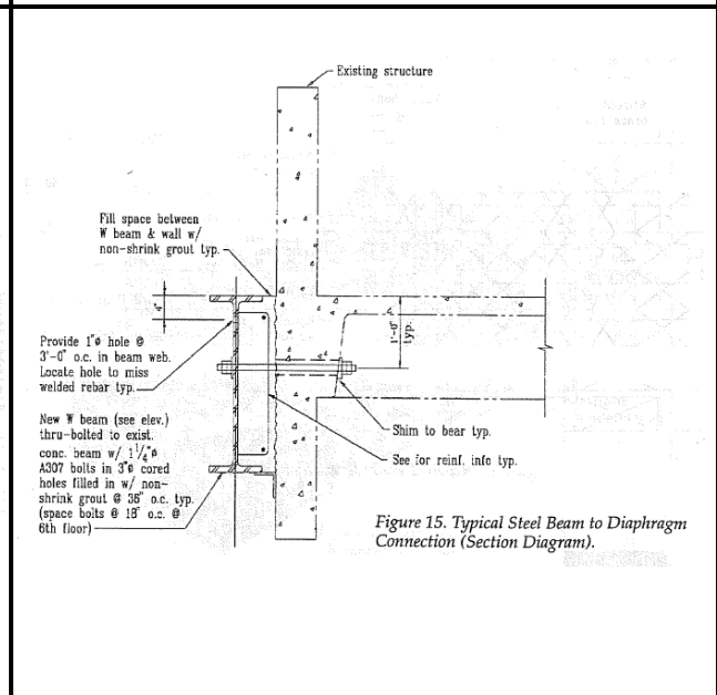
Typical steel beam to diaphragm connection. (SSC, 1994)
