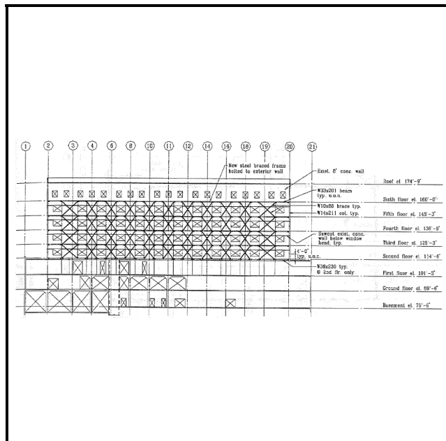
Repaired wall elevation at Line G. (SSC, 1994)
