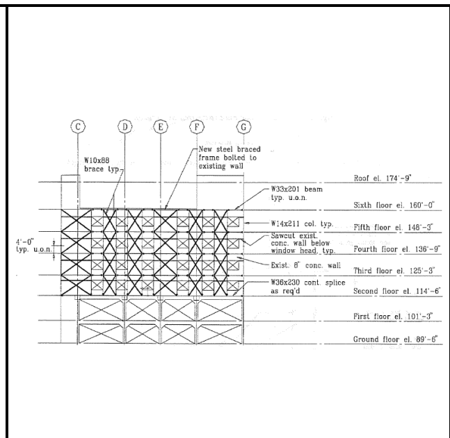
Repaired wall elevation at Line 20. (SSC, 1994)
