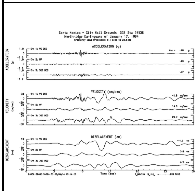
Ground acceleration, velocity and displacement at CSMIP Station No. 24538. (CESMD, 1994)
