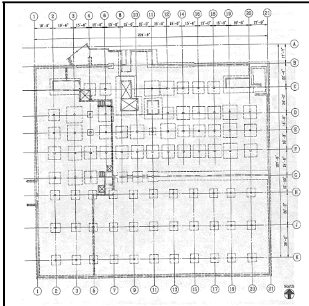
Foundation plan. (SSC, 1994)
