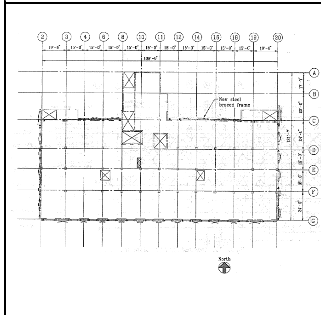
Typical floor plan of repaired structure. (SSC, 1994)
