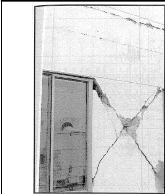
Typical shear wall damage. (SSC, 1994)
